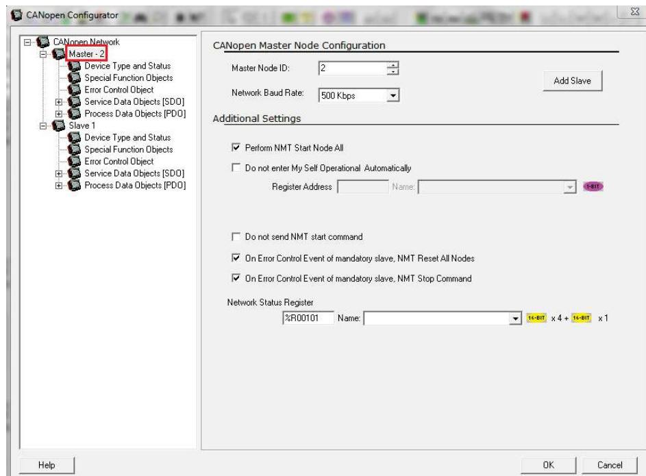
Figure 4-6. CANopen Configurator – Master
