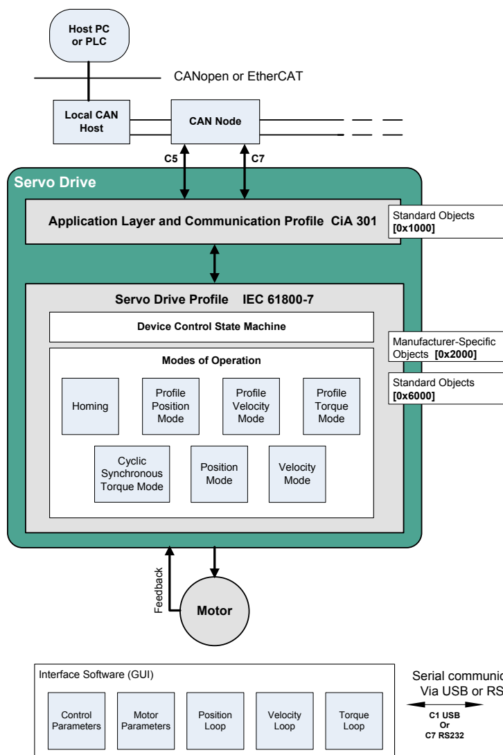
Figure 7-1. Communication Architecture
