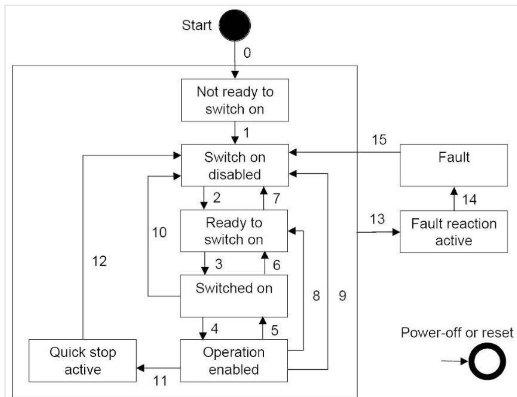
Figure 7-3. Power Drive System State Diagram
